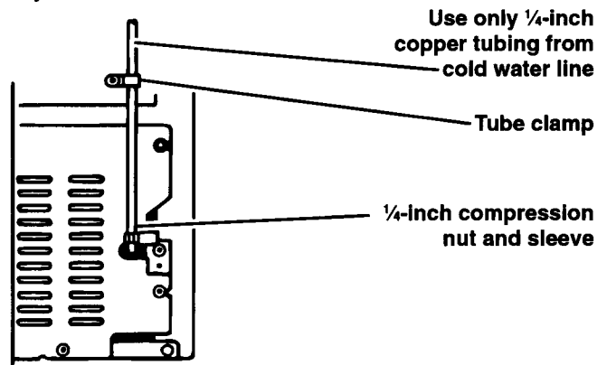
Style #2 valve
