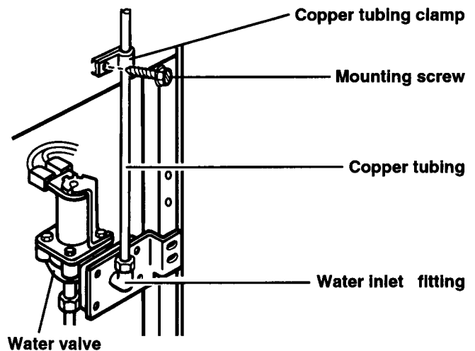
Style #2 valve
